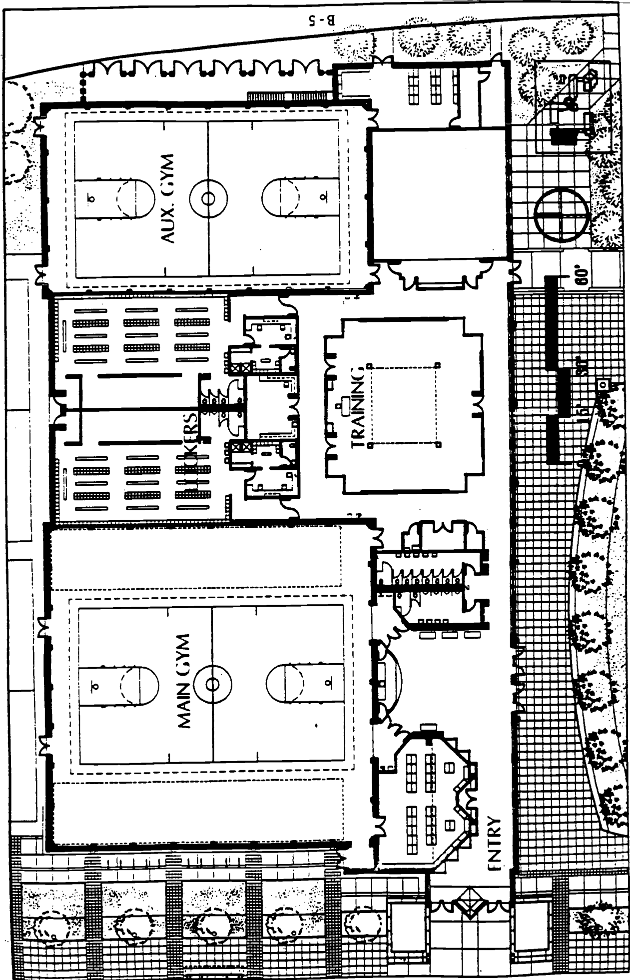
GYM COMPLEX
